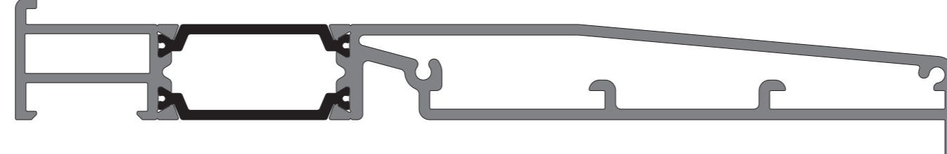
KAS 629 175mm Cill
