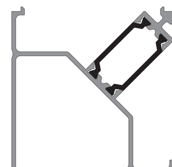
KAS 614 70mm Corner Post
