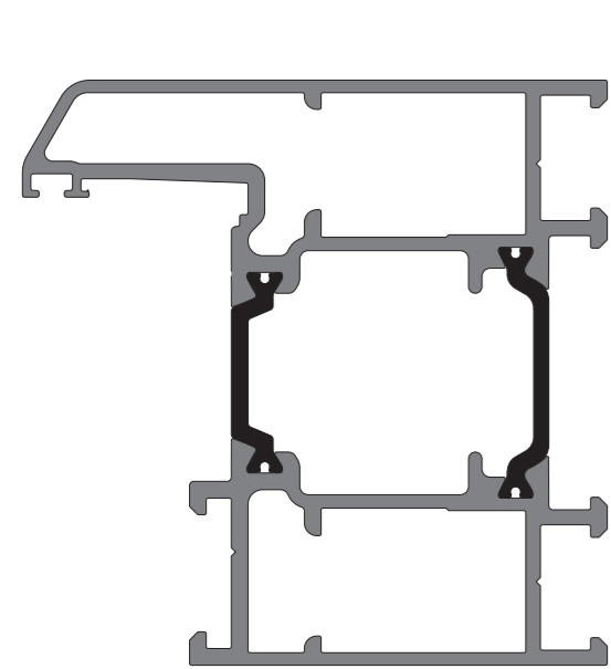
KAS 732 Stile / Rail Section
